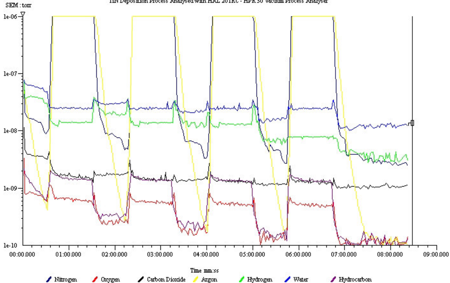
TiN Deposition Process Analysed with HAL 201RC - HPR 30 Vacuum Process Analyser
